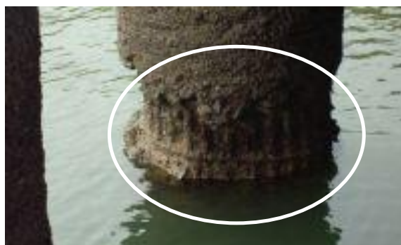
Figure 1.4. Prestressed concrete marine pile with spalling and reinforcement corrosion in a marine environment (Port Strategy 2007)
