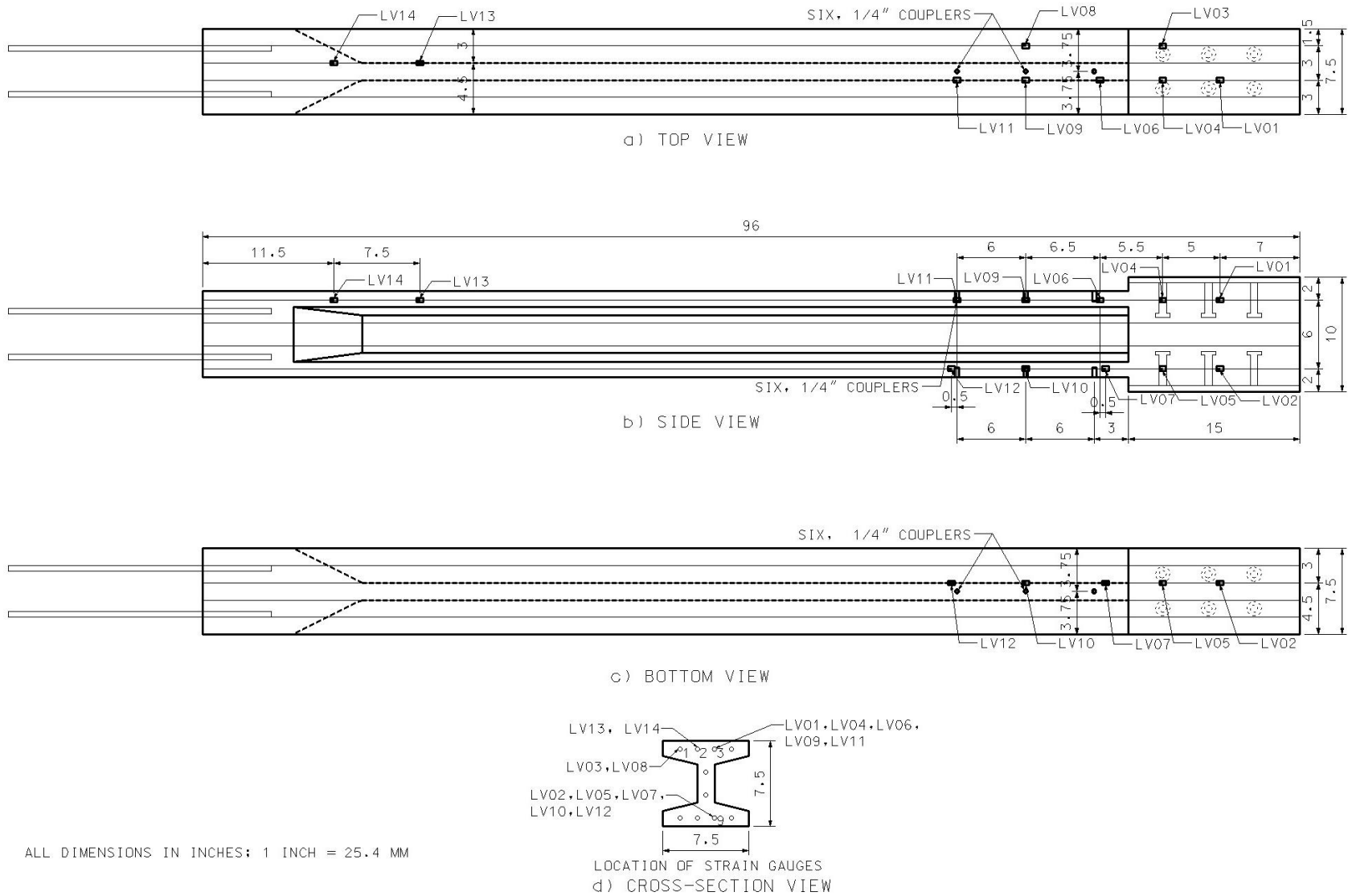
Figure 4.5. Details of instrumentation used for 8-ft (2.4-m) long UHPC laboratory test unit L1
