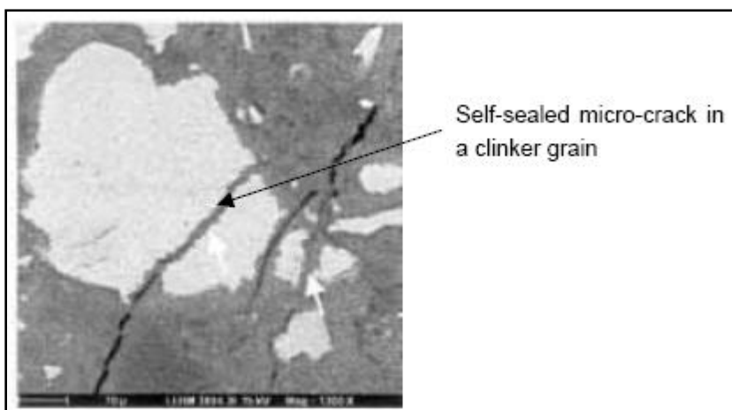
Figure 2.7. Self-healing of UHPC micro-crack (Acker and Behloul 2004)
