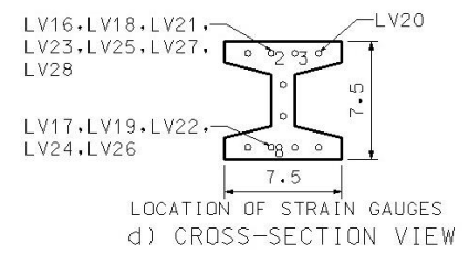
Figure 4.6. Details of instrumentation used for 8-ft (2.4-m) long UHPC laboratory test unit L2
