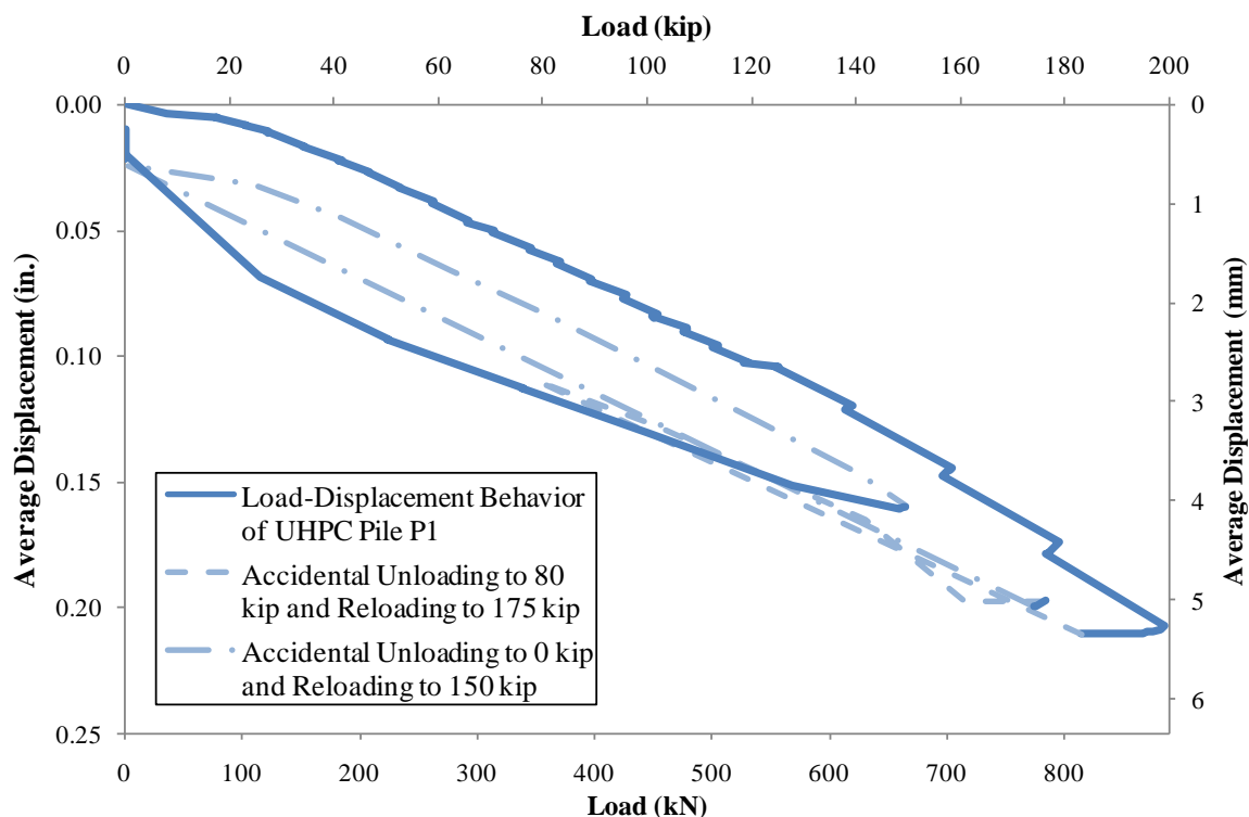
Figure 5.22. Observed load-displacement behavior for UHPC pile P1 during vertical load test 1
