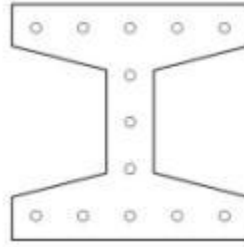
Figure 3.6. Tapered H-shaped section considered for UHPC pile
